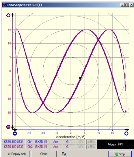
Orbital mode: display movements of the measurement object in the plane
